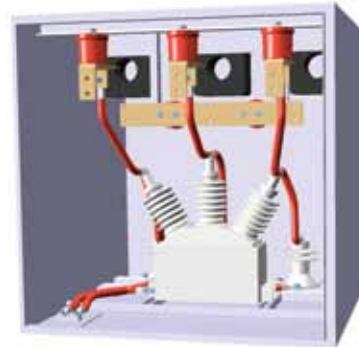
Main Terminal Box with Optional Accessories
