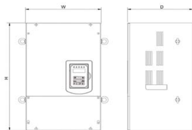
D 50-100 HP, 230V/ 100-200 HP, 460V (IP00) 100-250 HP, 690V (IP00)
