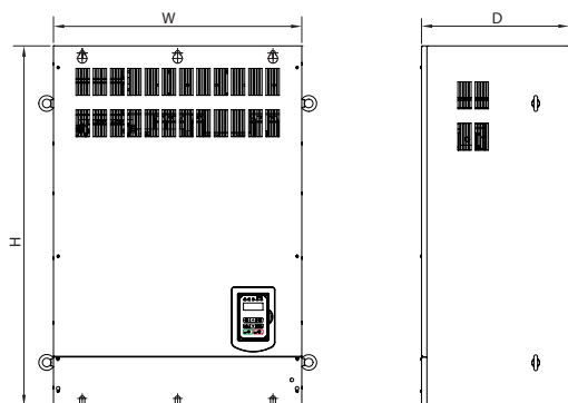
E 250-400 HP, 460V (IP20/ NEMA 1)
