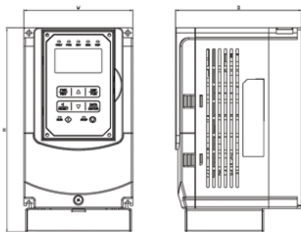
A 1-7.5 HP, 230V/ 1-7.5 HP, 460V (IP20/ NEMA 1) 1-3 HP, 575V (IP20/ NEMA 1)
