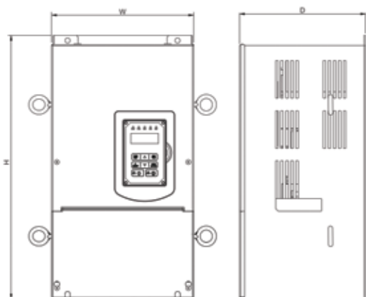
C 30-40 HP, 230V/ 40-75 HP, 460V (IP20/ NEMA 1) 50-75 HP, 690V (IP20/ NEMA 1)
