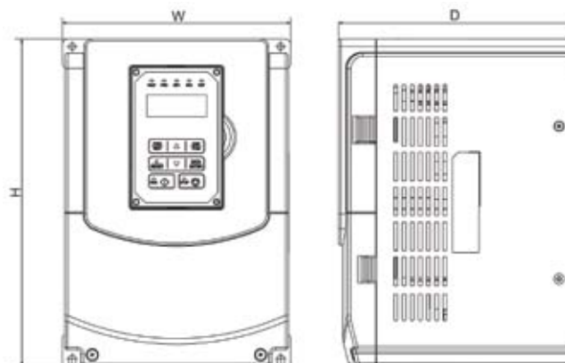
B 10-25 HP, 230V/ 10-30 HP, 460V (IP20/ NEMA 1) 5-10 HP, 575V/ 15-40 HP, 690V (IP20/ NEMA 1)
